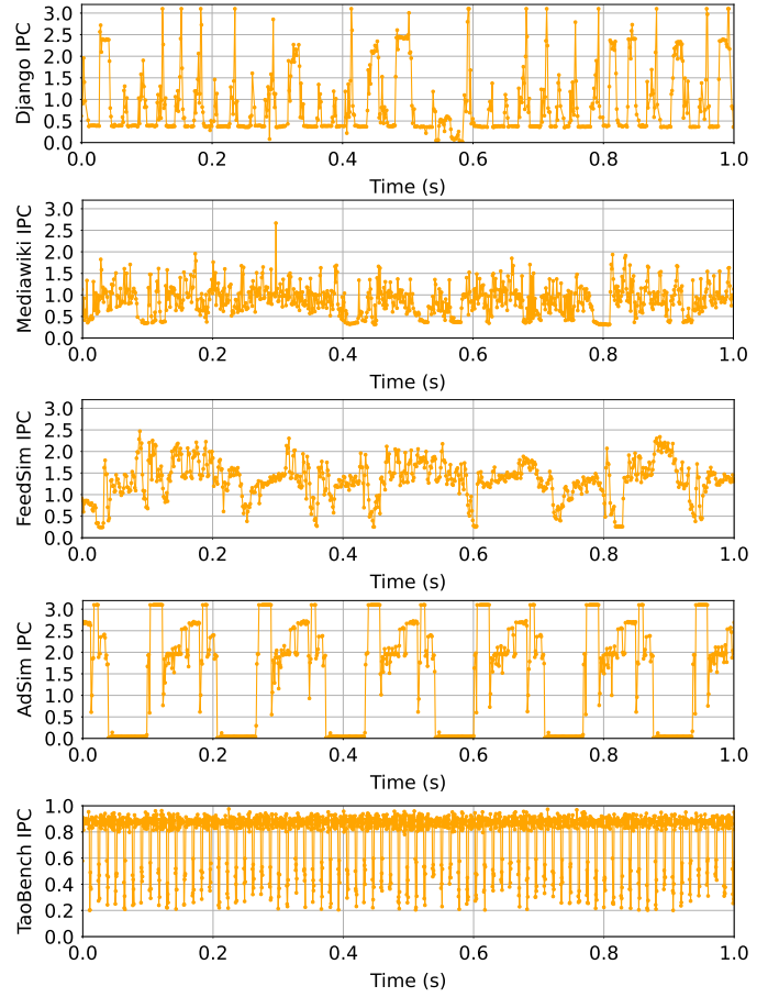
Fig. 2: IPC over time for different DCPperf workloads: Django , Mediawiki , FeedSim , AdSim , and TaoBench .
